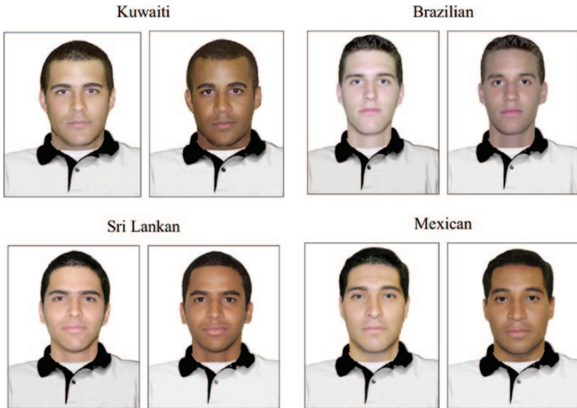
Figure 1. The Afrocentric Manipulation.
