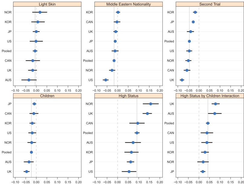
Figure 4. A Comparison of the Pooled and Within-Country Effects. Plotted points are maximum likelihood estimates of the indicated regression parameters, by country or pooled across countries. Horizontal lines cover 95-percent confidence intervals; in some cases, these are so narrow as to be obscured by the plotted point. A dotted vertical line indicates zero; the solid vertical line indicates the pooled estimate.
