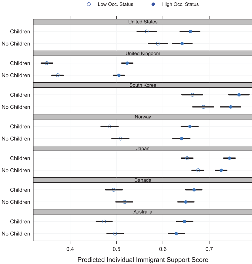
Figure 3. Interaction Effects of Occupational Status and Dependents Manipulations. Plotted points are predicted values of the individual immigrant support score, varying the high/low occupational status and children/no-children conditions, by country; the generalized immigrant support score is set at its country-specific mean, the trial indicator is set to the first trial, and we assume that the hypothetical, individual immigrant is not of Middle Eastern origin. Open/solid plotting symbols indicate low/high occupational status. Horizontal lines cover 95-percent confidence intervals around the predicted values.
