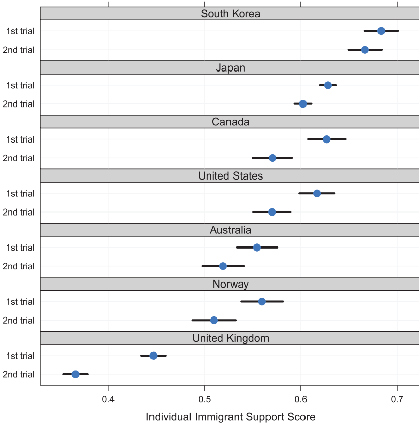
Figure 2. Cross-National Differences in Evaluations of Individual Immigrants. Plotted points are the observed, average values of the individual immigrant support score, by country, by trial. Horizontal lines cover 95-percent confidence intervals for each average score.
